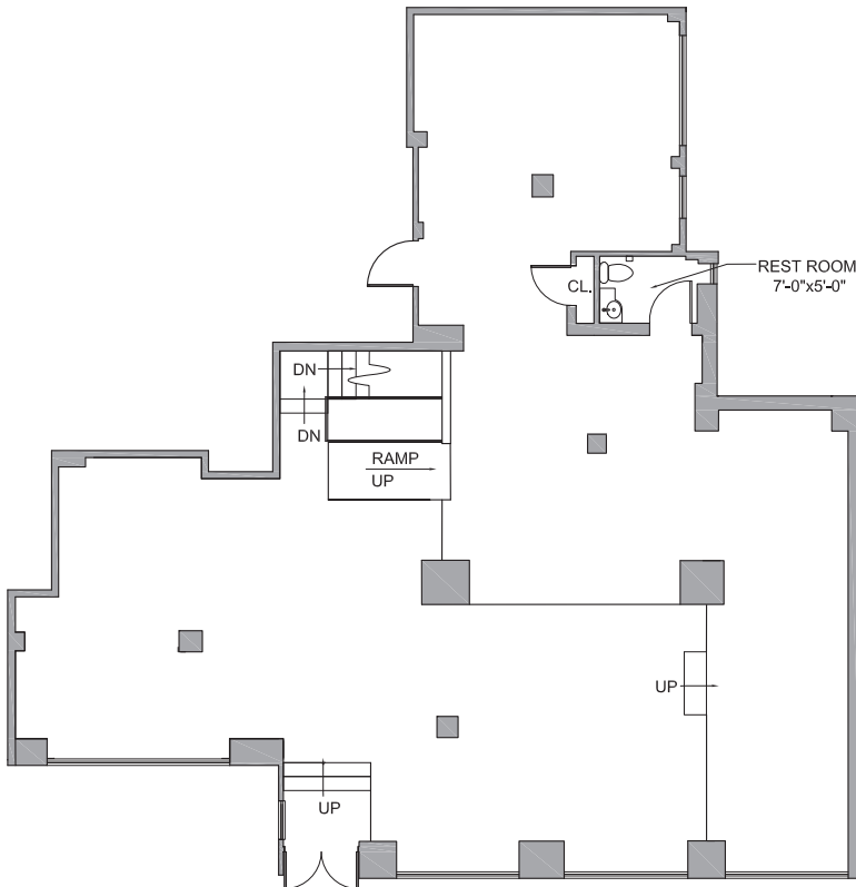
GROUND
